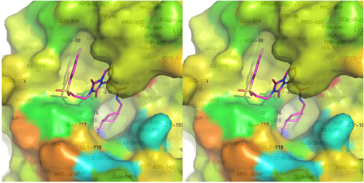
C_thrombin-diff-elec-coeff_thr-try.png
