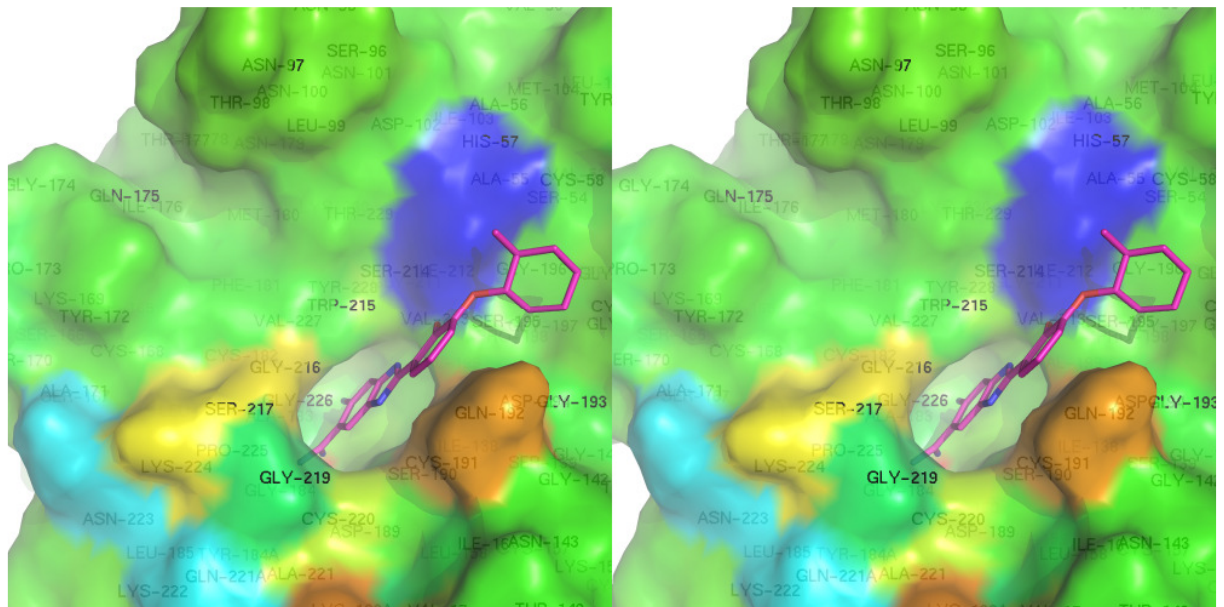
B_trypsin-diff-elec-coeff_try-thr.png
