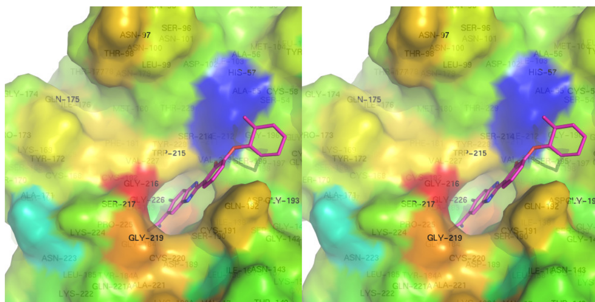
B_trypsin_elec-PLS-coeff.png
