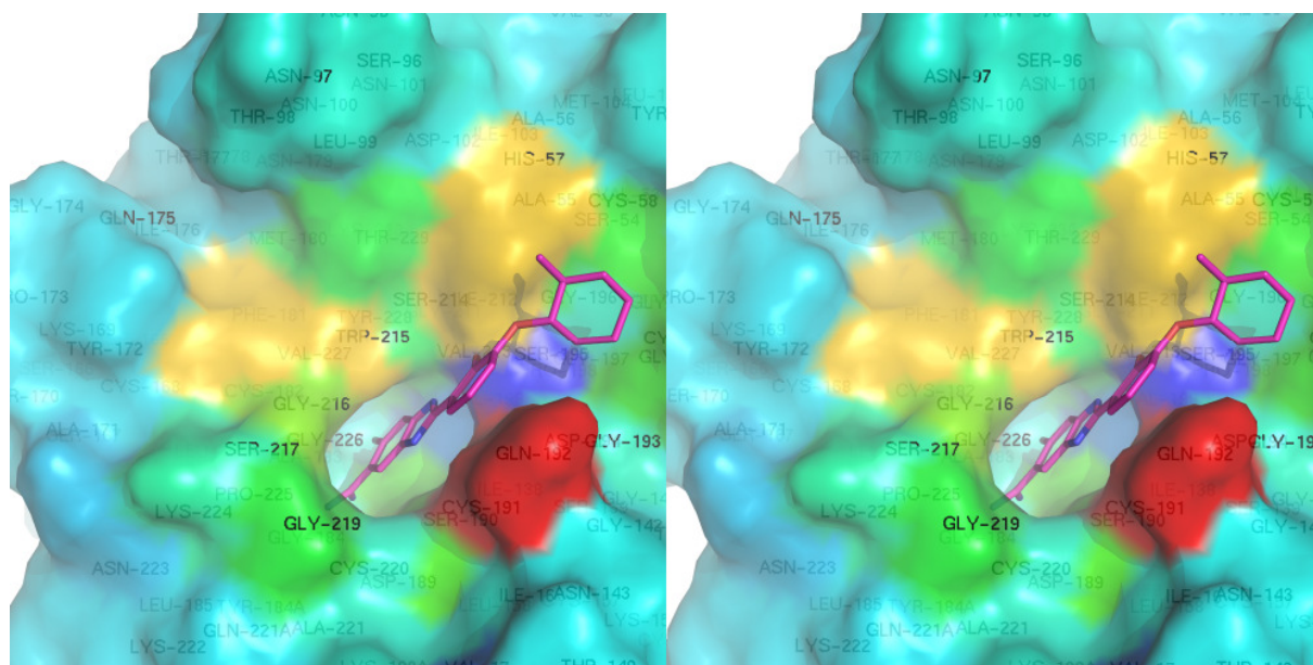
B_trypsin_vdw-PLS-coeff.png
