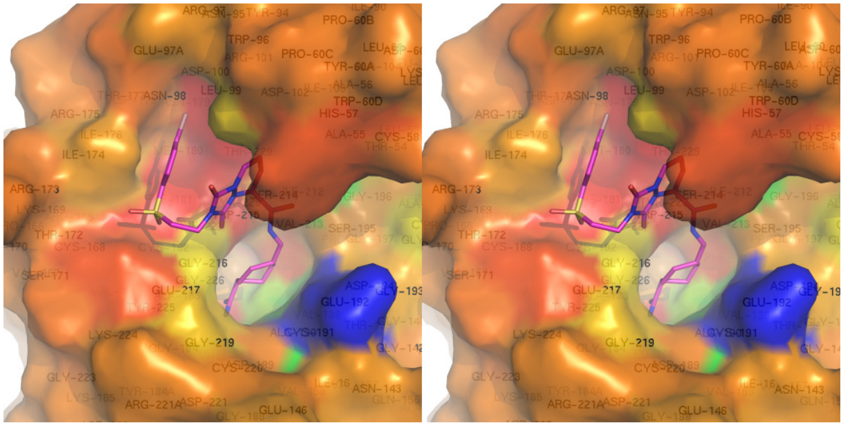
C_thrombin-diff-vdw-coeff_thr-try.png
