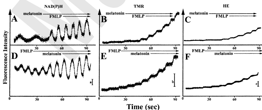
FIGURE 10 The effects of melatonin (50 \mu M) and FMLP (50 nM) on NAD(P)H oscillations and oxidant release. ( A ) Although melatonin alone has no effect on NAD(P)H oscillations, when FMLP is added to the cells both the frequency and amplitude of the oscillations are increased. ( B and C ) The production of oxidants as detected by tetramethylrhodamine and EB formation are dramatically enhanced in the presence of melatonin and FMLP. ( D ) As noted in Fig. 7, FMLP increases the frequency of NAD(P)H oscillations. When melatonin is added, the amplitude increases. ( E and F ) The production of oxidants is enhanced by FMLP and further enhanced when melatonin is added.
